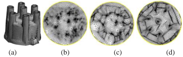
Figure 2: (a) Input triangulation, parameterization with (b) constant, (c) least-square, and (d) shape-preserving weights.
