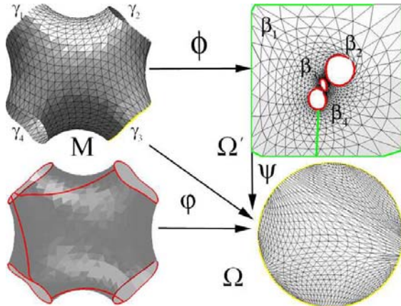
Figure 3: General framework for the parameterization of a surface patch with k = 4 boundary components.
