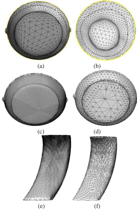
Figure 10: (a) Input conical primitive, (b) shape-preserving parameterization; (c) regular and (d) adaptive remesh of (a). The examples (e) and (f) show the uniform and adaptive remesh of the cylinder in Figure 4.
